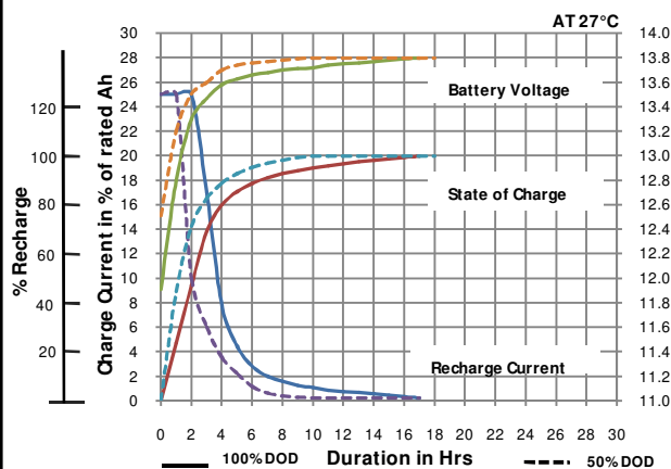
CONSTANT VOLTAGE CHARGING CHARACTERISTICS
